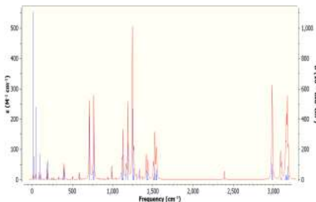
3.2-rasm. Bisbuteronitrildiaminning DFT IQ-spektri
